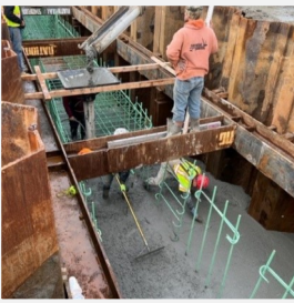
Rehabilitation of Seawall Route 146, Limewood Avenue Branford, Connecticut
